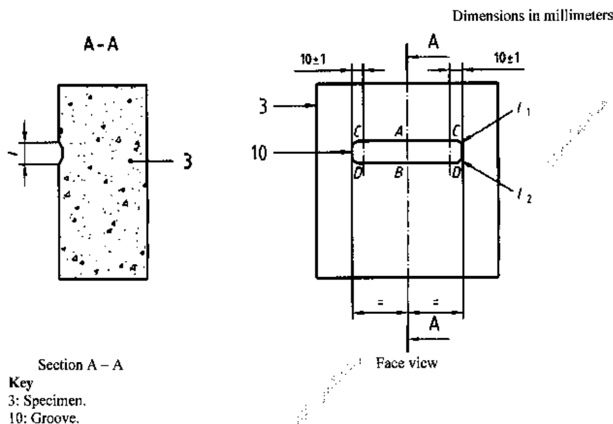
Figure 8 — Example of a tested specimen showing a groove
