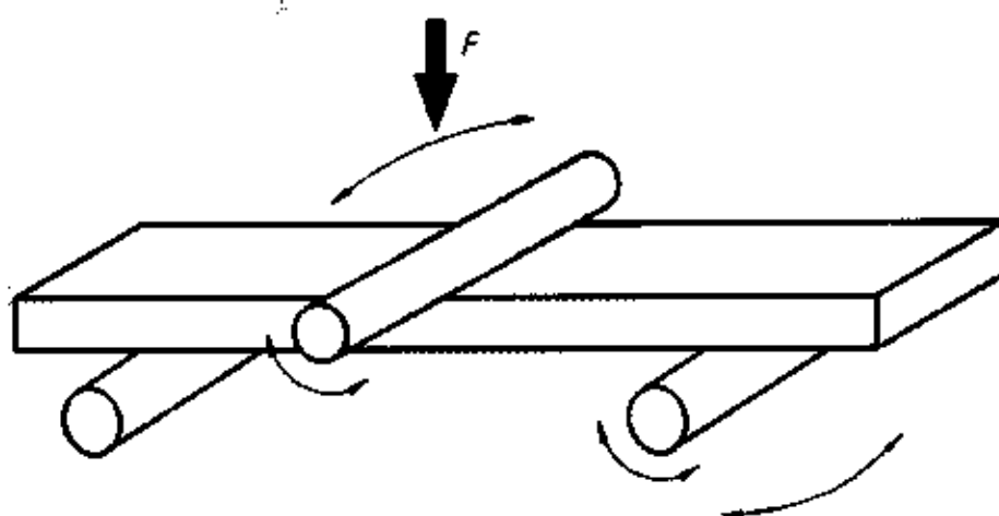
Figure 4 — Principle of testing
