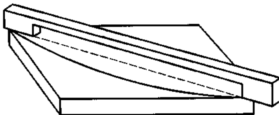
Figure 3 — Measurement of upper face flatness
