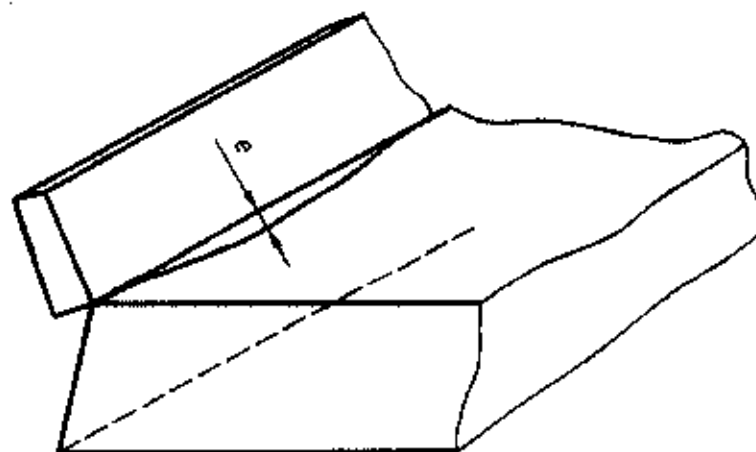
Figure 2 — Measurement of edge straightness
